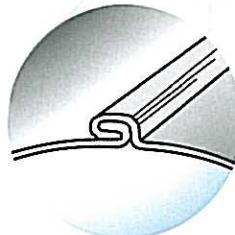
4 - Ply Lock Seam
